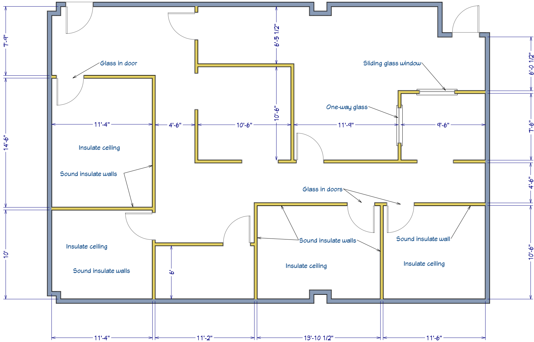
BASEMENT OFFICE SPACE
